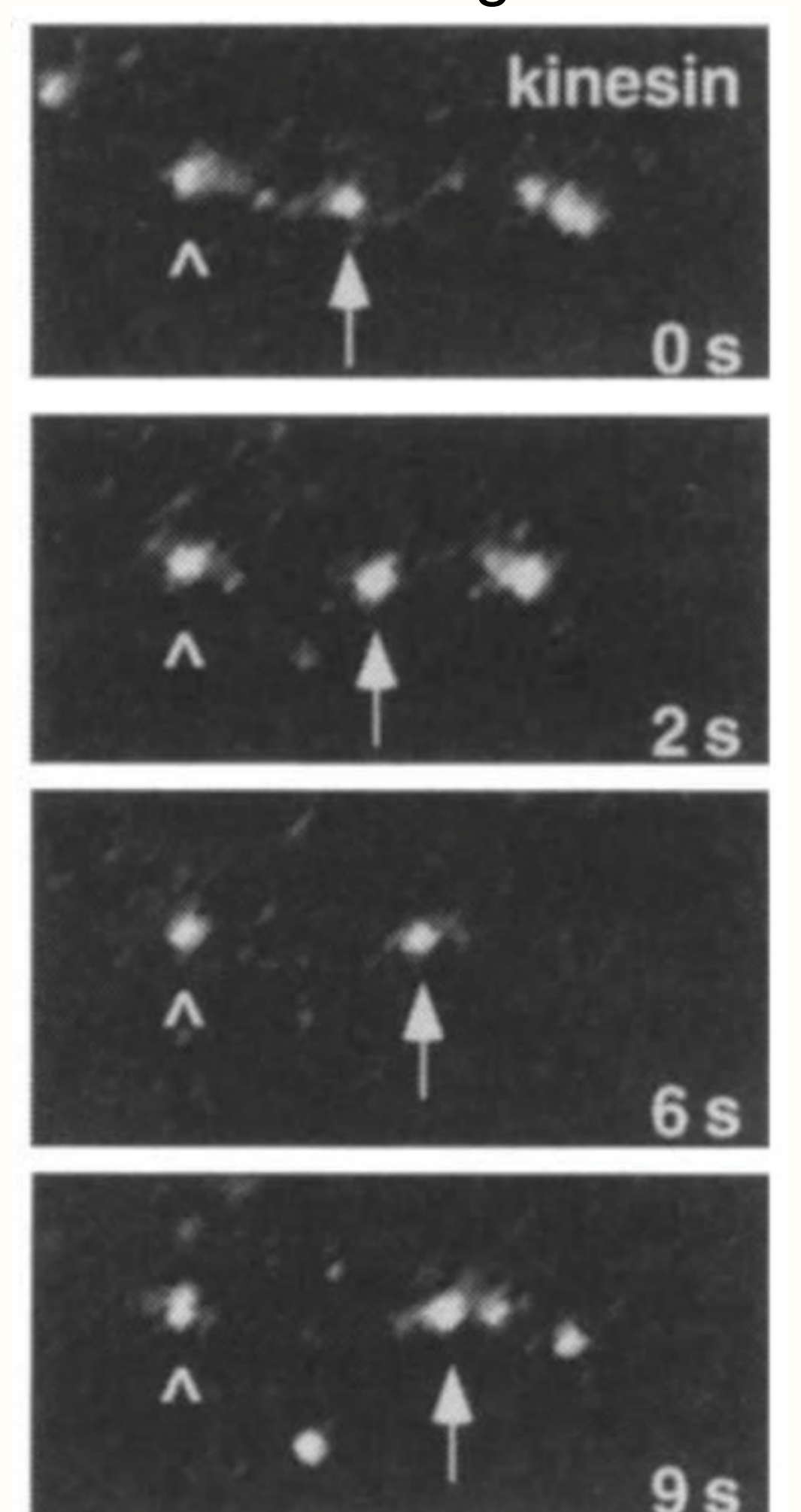
Kinesin moving Vale et. al. 1996
